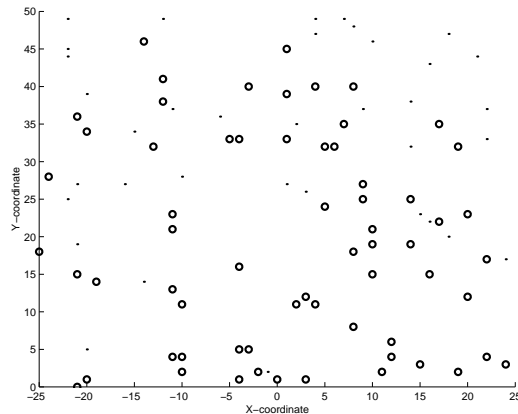
Figure 12. Sensors that remain alive (circles) and those that are dead (dots) after 1200 rounds with 0.5 J/node for LEACH. Note that this shows the network 1020 rounds further along than Figure 6.
