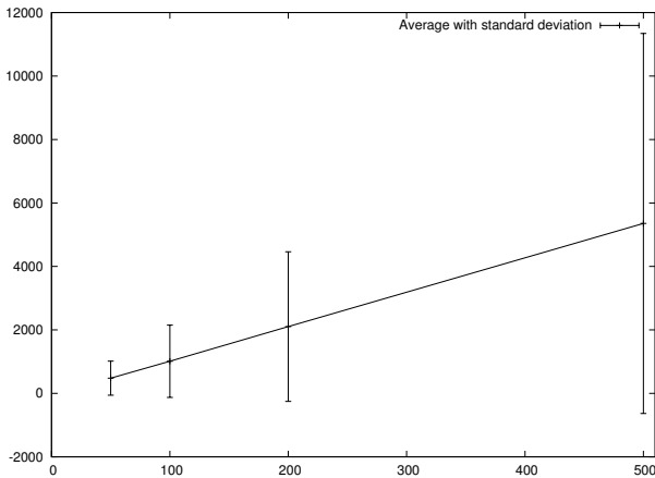
Fig. 6. Number of broadcast messages sent to build the topology.
