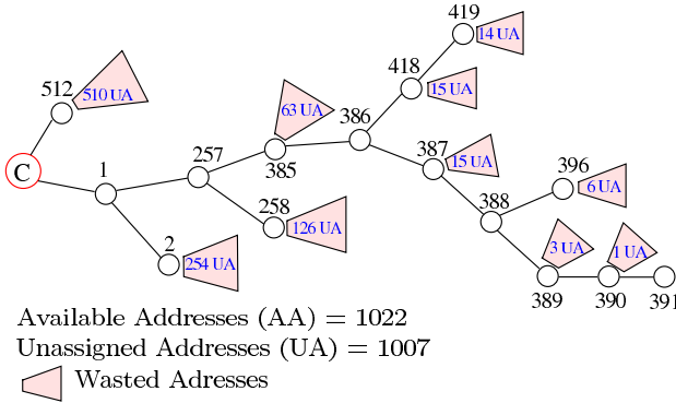
Fig. 1. Waste of addresses on a ZigBee cluster-tree ( Rm=2 , Cm=2 , Lm=9 ).
