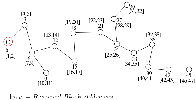
Fig. 12. Simple topology discovered by TopoProto
