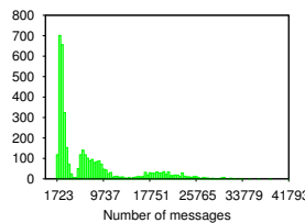
Fig. 11. Distribution of total number of unicasts for various 500 nodes topologies.
