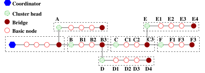
Fig. 2. A Long Thin WSN as proposed in [9]
