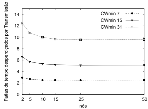
(b) backoff .
