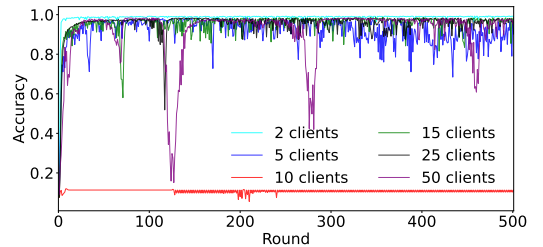
Fig. 3. Baseline FedAvg classification accuracy on MNIST under non-IID partitioning across client pool sizes.
