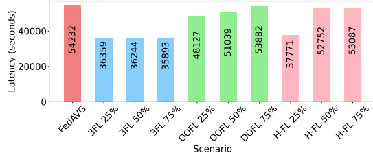
(b) Cumulative latency on CIFAR-10.
