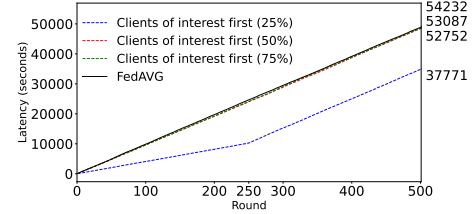
(b) CIFAR-10 latency profile.
