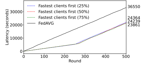
(a) Cumulative latency on MNIST.
