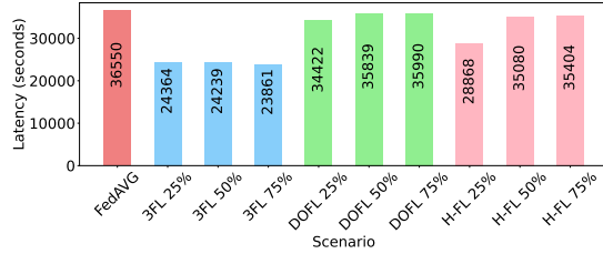
(a) Cumulative latency on MNIST.
