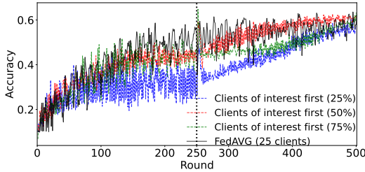
(b) CIFAR-10 accuracy trajectory.
