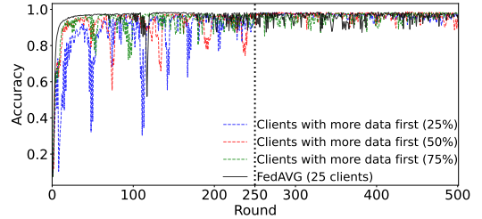
(a) MNIST accuracy trajectory.
