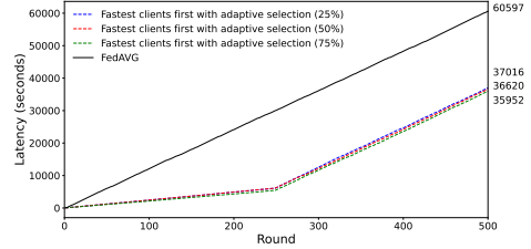
Fig. 9. A-3FL cumulative training latency under time-varying straggler probabilities on MNIST.
