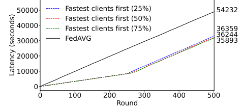
(b) Cumulative latency on CIFAR-10.
