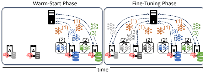
Fig. 1. 3FL: Fast devices (“B”) complete the calibration phase to build a warm-start model before slower devices (“A”) join for full-data fine-tuning.
