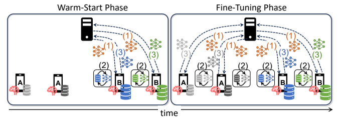
Fig. 2. DOFL scheme: Clients holding larger datasets (“B”) are prioritized during early rounds to maximize information density before full federation.
