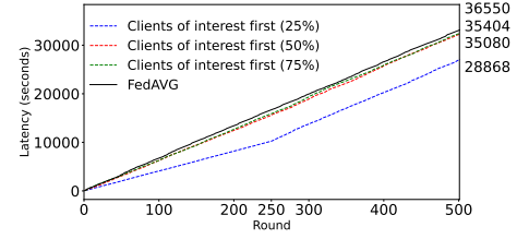
(a) MNIST latency profile.
