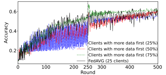
(b) CIFAR-10 accuracy trajectory.
