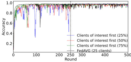
(a) MNIST accuracy trajectory.
