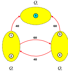
(a) An admissible flow network from Phase I for super-sensors Q_1 and Q_2 with base station in Q_3 .
