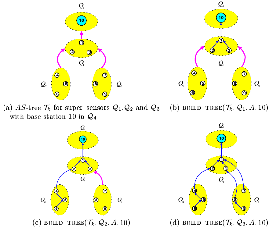
Figure 5: Illustration of the BUILD-TREE procedure for an AS-tree \mathcal{T}_k . Sensors 1, 2, \dots , 9 are partitioned among super-sensors \mathcal{Q}_1, \mathcal{Q}_2 , and \mathcal{Q}_3 . Super-sensor \mathcal{Q}_4 contains the base station 10. The aggregation tree A is used for collecting one data packet from each sensor and transmitting to the base station.
