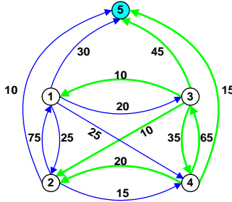
(c) The INCREMENTAL CMLDA flow network for the sensors with lifetime of 100 rounds.
