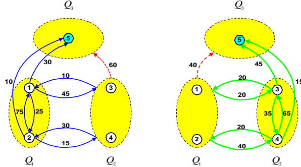
(b) Capacity provisioning from Phase II for sensors 1, 2 in super-sensor Q_1 and sensors 3, 4 in super-sensor Q_2 .
