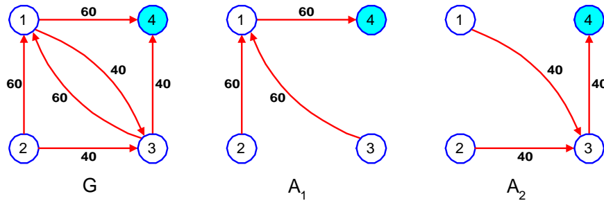
Figure 1: An admissible flow network G with lifetime 100 rounds, and two aggregation trees A_1 and A_2 with lifetimes 60 and 40 rounds respectively.
