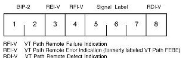
Figure 10. VT Path Overhead -- V5 Byte
