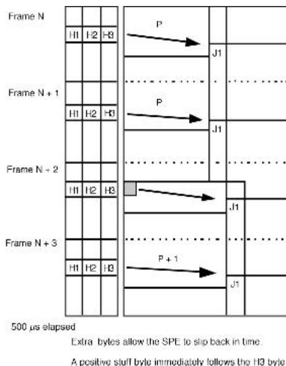
Figure 12. Payload Pointer Positive Justification
