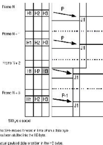
Figure 13. Payload Pointer Negative Justification
