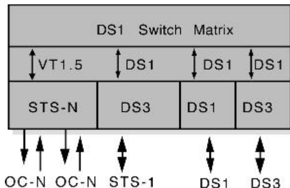
Figure 23. Wideband Digital Cross-Connect
