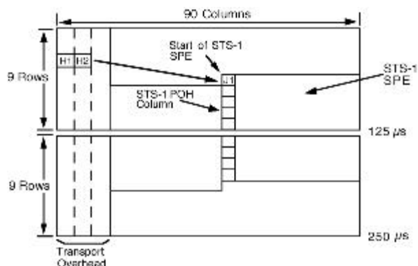
Figure 11. Pointer SPE Position in the STS-1 Frame
