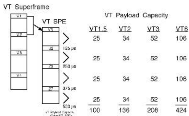
Figure 18. VT SPE and Payload Capacity
