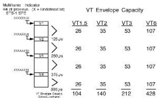
Figure 17. VT Superframe and Envelope Capacity
