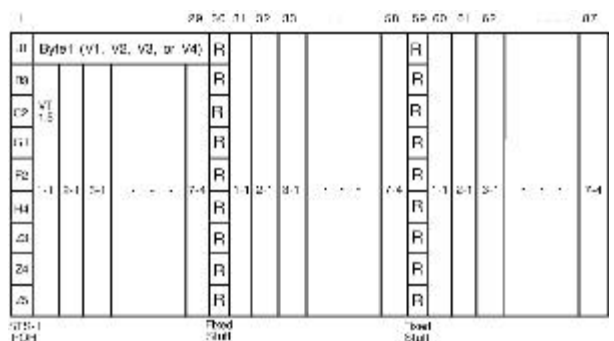
Figure 16. STS-1 VT1.5 SPE Columns
