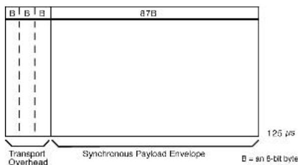
Figure 1. STS-1 frame format
