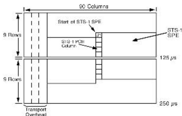
Figure 4. STS-1 SPE Position in the STS-1 Frame
