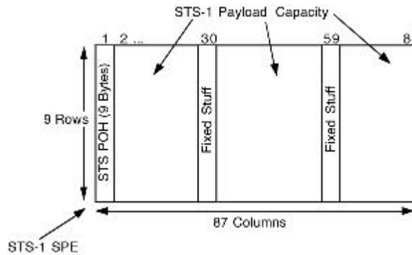
Figure 3. STS-1 SPE example
