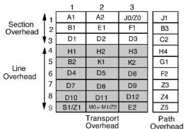
Figure 8. Line Overhead - Rows 4 to 9 of Transport Overhead
