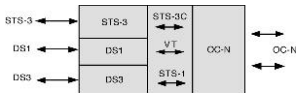
Figure 20. Terminal Multiplexer
