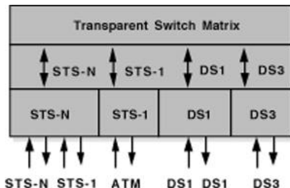
Figure 24. Broadband Digital Cross-Connect
