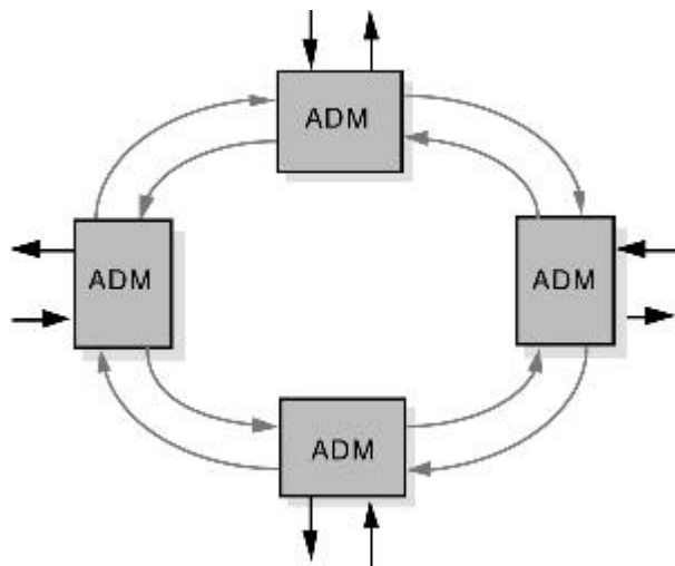
Figure 29. Ring Architecture
