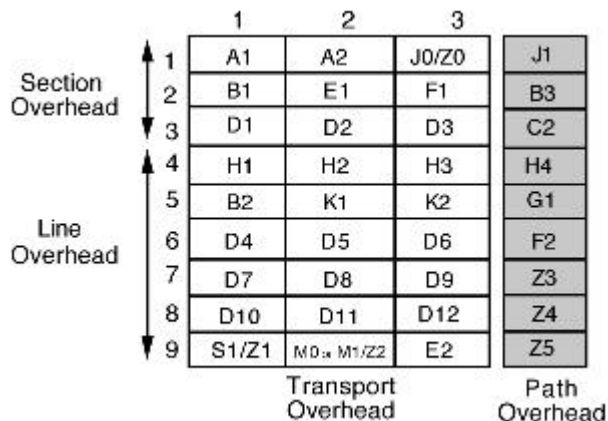
Figure 9. Path Overhead - Rows 1 to 9
