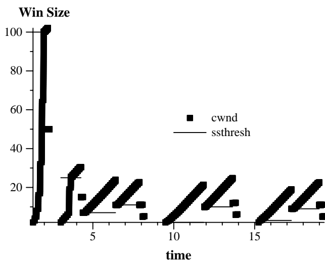
Congestion Window 9 (Reno_10_flows)
