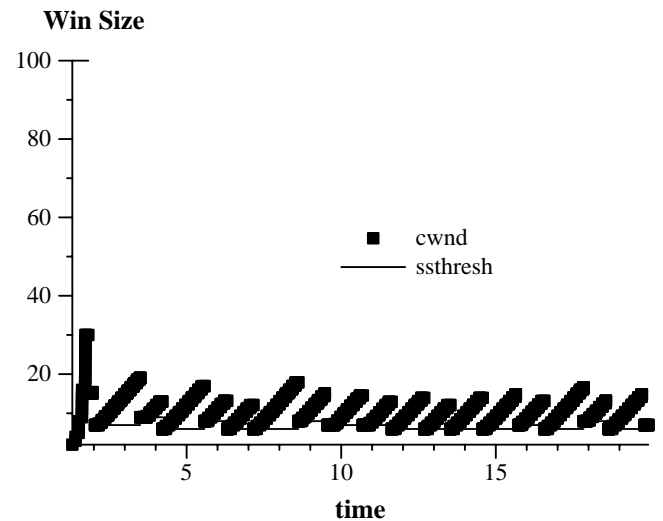
Congestion Window 9 (Sack_10_flows)
