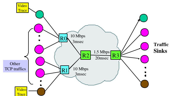
Figure 7: Network Model for Simulation.
