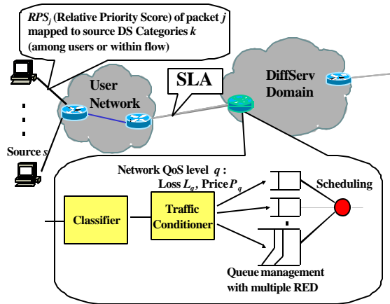
Figure 1: Overall framework of proposed content-based packet video forwarding.
