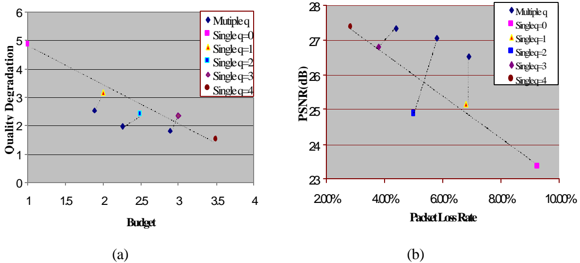
Figure 9: The performance comparison of the ‘Foreman’ sequence under multiple-queue scenario: (a) the quality degradation vs. the pricing budget, and (b) end-to-end video quality vs. network packet loss.
