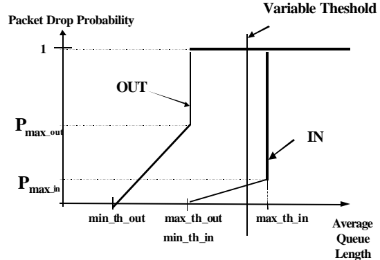
Figure 4: Control parameters of RIO queuing.
