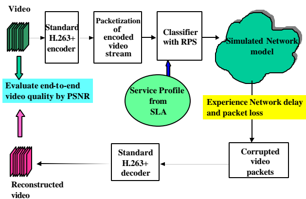
Figure 6: The overall simulation diagram for video applications in a DiffServ Network.
