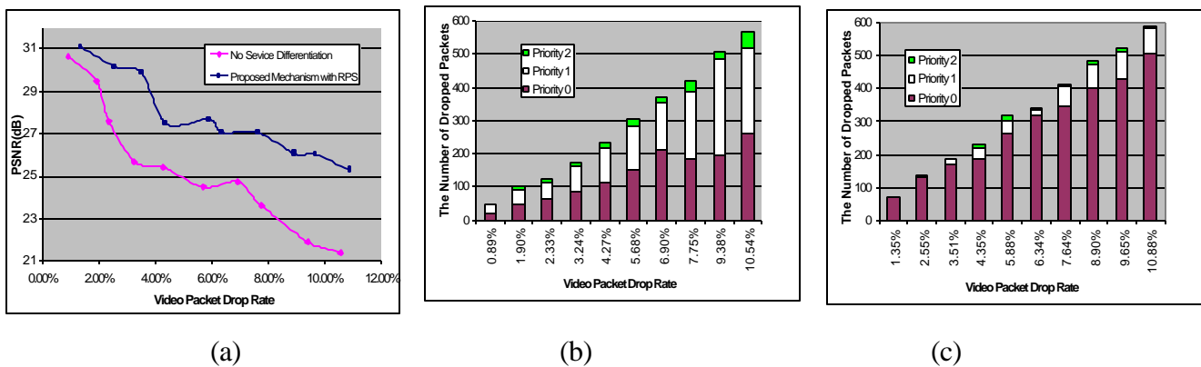
Figure 8: The performance comparison of the ‘Foreman’ sequence under the single queue scenario: (a) the video packet drop rate vs. the average PSNR for 300 frames. The number of dropped video packets in a network with (b) no service differentiation and (c) the proposed mechanism with RPS, where the total packet numbers/average byte of each class are 2675/205.8, 2381/204.5 and 351/243.2 for priority classes 0, 1 and 2, respectively.
